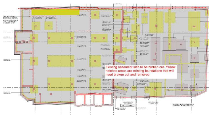
Extend of existing foundations
